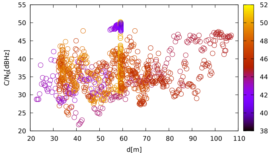
C/N 0 vs distance (JavadLSA at C 1 for G03 at L1)
