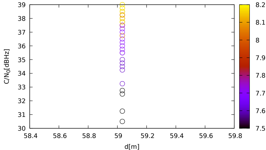
C/N 0 vs distance (JavadLSA at C 1 for G04 at L1)
