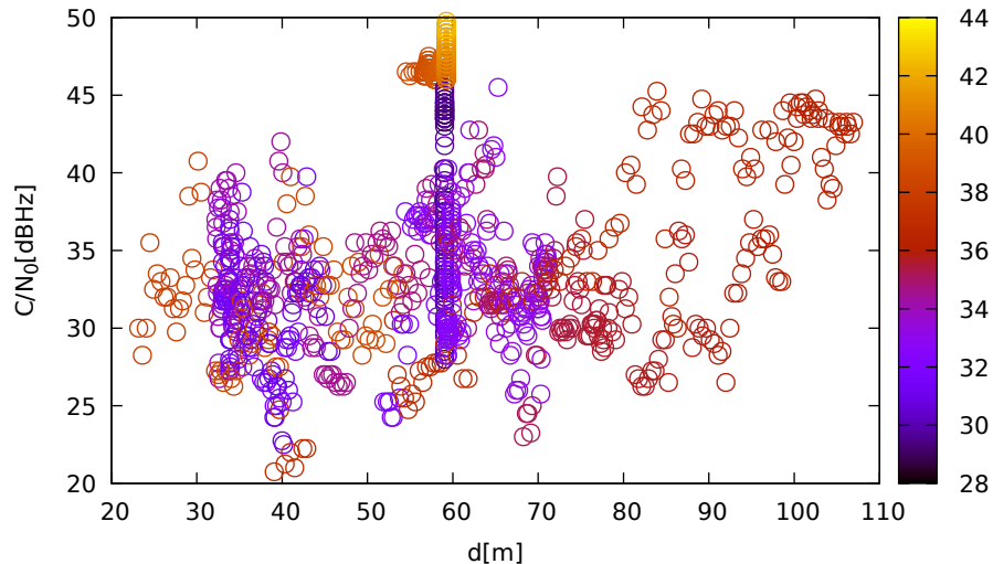
C/N 0 vs distance (JavadLSA at C 1 for G08 at L1)
