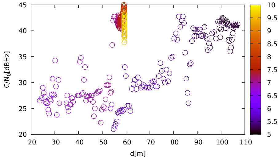
C/N 0 vs distance (JavadLSA at C 1 for G10 at L1)
