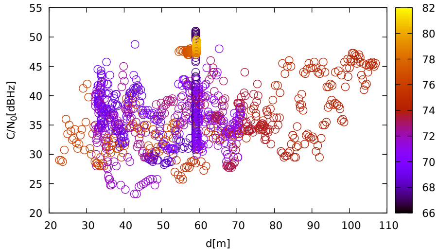
C/N 0 vs distance (JavadLSA at C 1 for G11 at L1)
