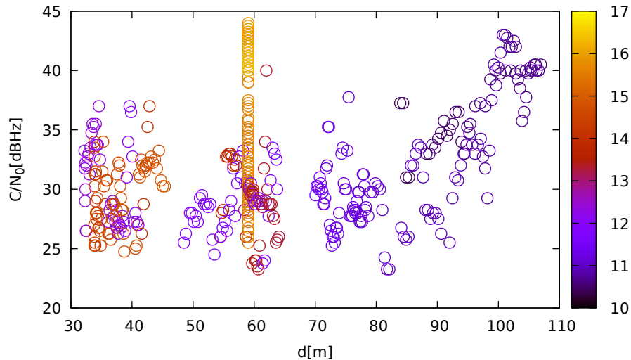
C/N 0 vs distance (JavadLSA at C 1 for G17 at L1)
