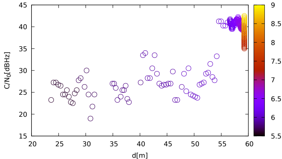
C/N 0 vs distance (JavadLSA at C 1 for G21 at L1)
