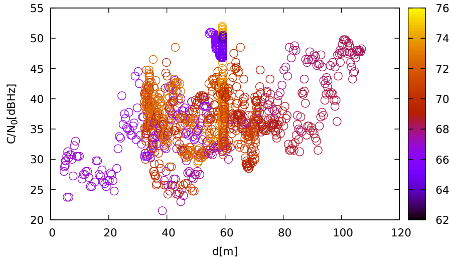
C/N 0 vs distance (JavadLSA at C 1 for G22 at L1)
