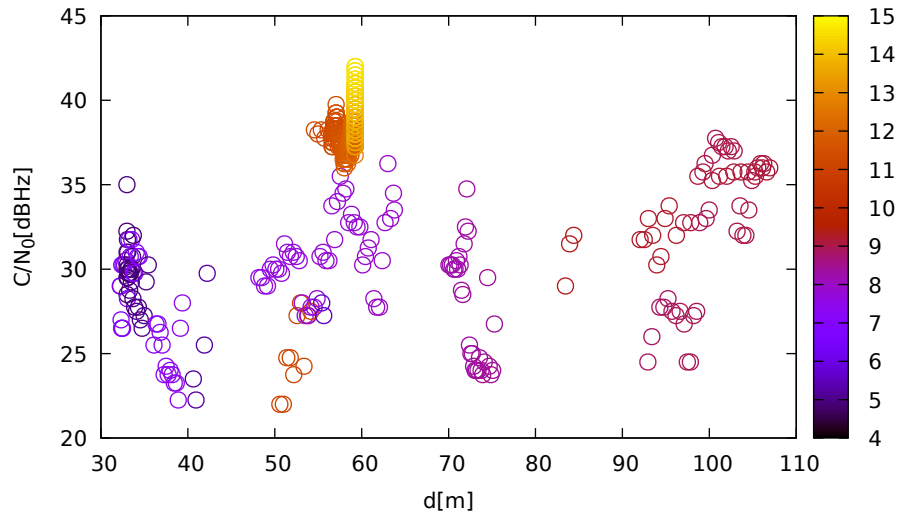
C/N 0 vs distance (JavadLSA at C 1 for G27 at L1)
