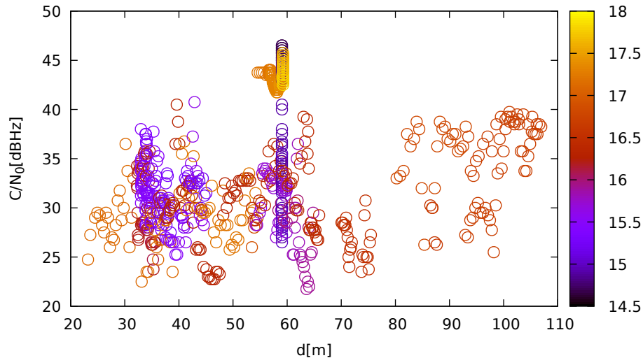
C/N 0 vs distance (JavadLSA at C 1 for G28 at L1)
