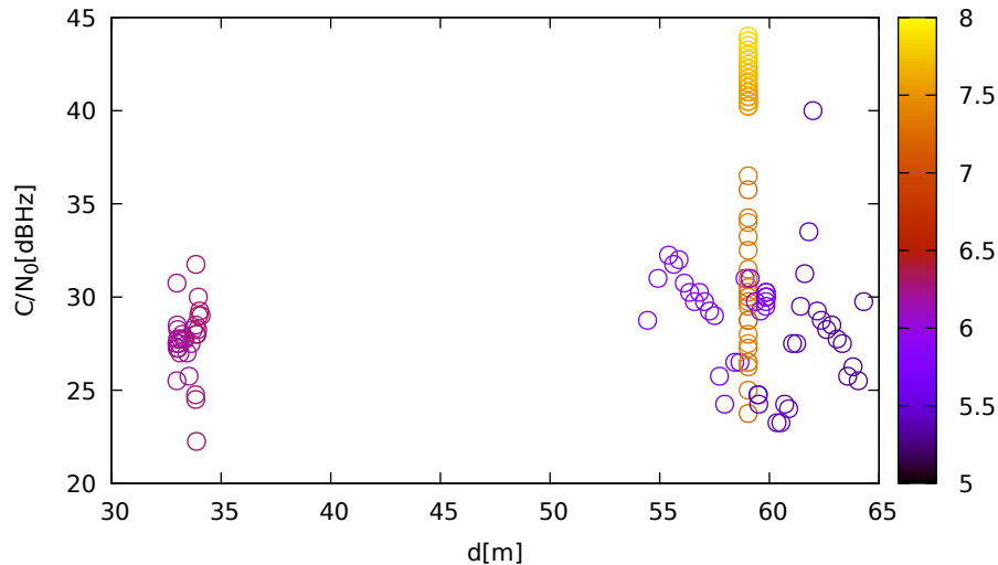
C/N 0 vs distance (JavadLSA at C 1 for G31 at L1)
