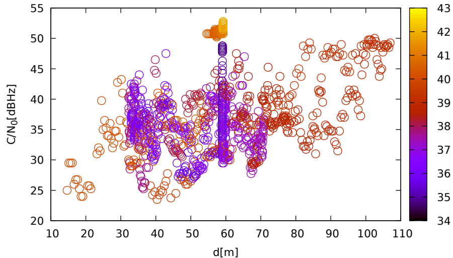
C/N 0 vs distance (JavadLSA at C 1 for G32 at L1)
