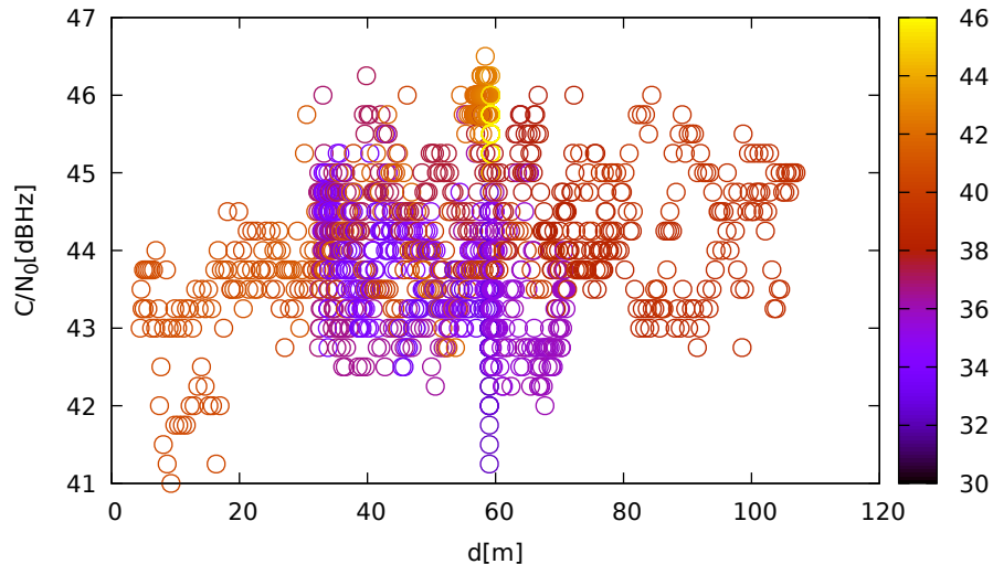
C/N 0 vs distance (JavadLSA at C 1 for R06 at L1)
