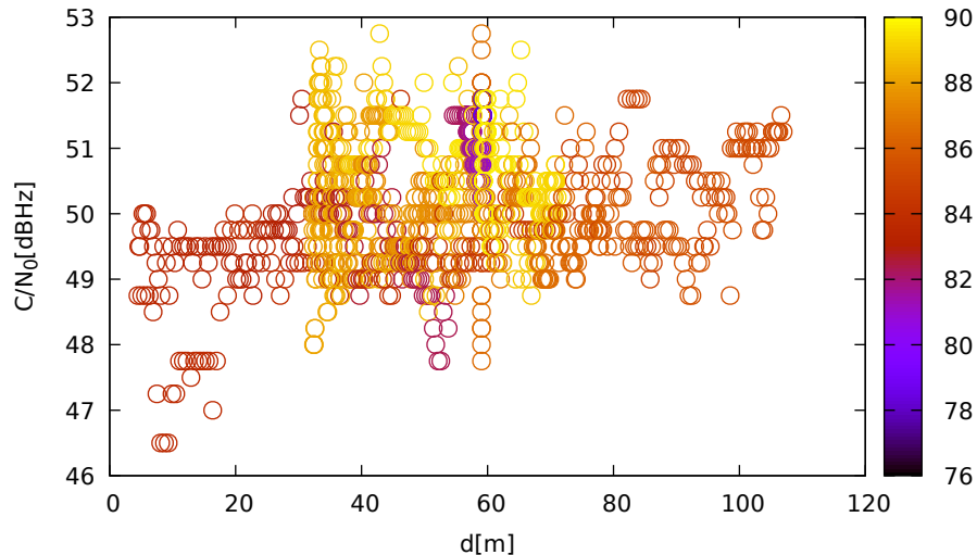
C/N 0 vs distance (JavadLSA at C 1 for R07 at L1)
