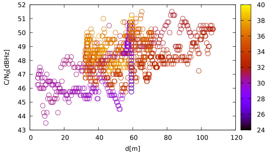
C/N 0 vs distance (JavadLSA at C 1 for R08 at L1)
