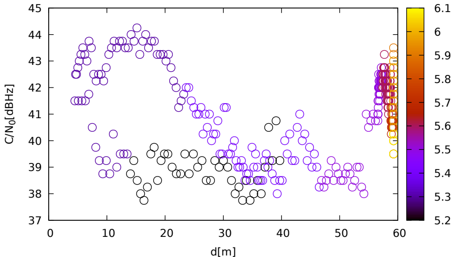
C/N 0 vs distance (JavadLSA at C 1 for R14 at L1)
