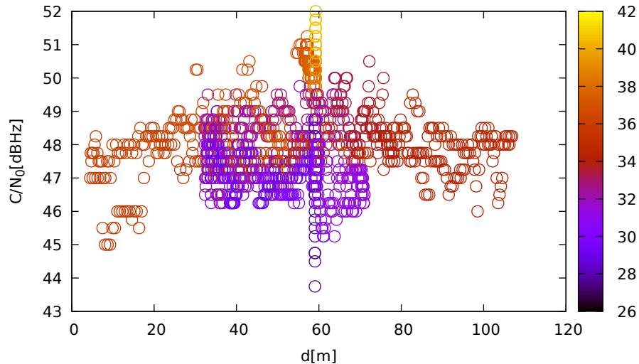
C/N 0 vs distance (JavadLSA at C 1 for R21 at L1)
