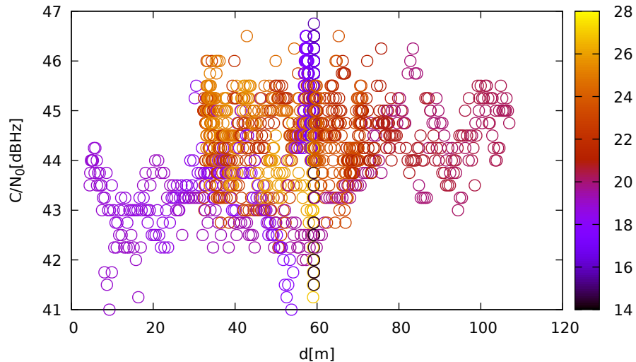
C/N 0 vs distance (JavadLSA at C 1 for R23 at L1)
