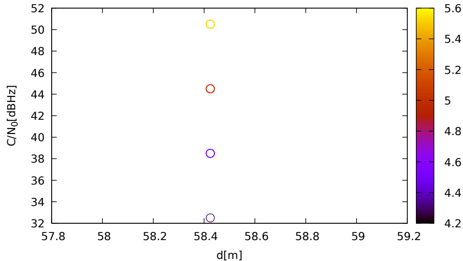
C/N 0 vs distance (LeicaGS15 at C 1 for E02 at L1)
