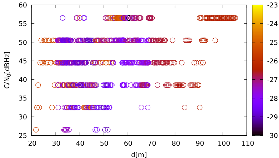
C/N 0 vs distance (LeicaGS15 at C 1 for E04 at L1)
