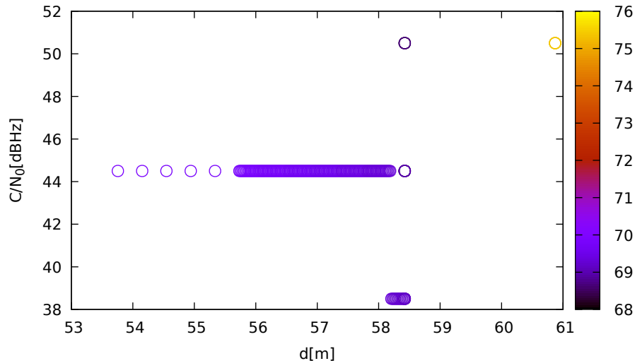
C/N 0 vs distance (LeicaGS15 at C 1 for E05 at L1)
