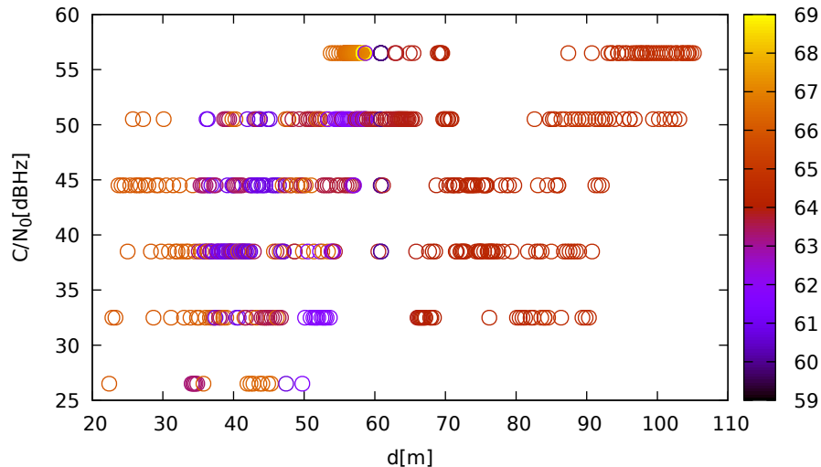
C/N 0 vs distance (LeicaGS15 at C 1 for E11 at L1)
