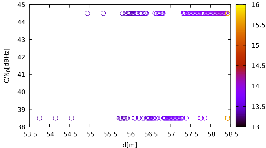
C/N 0 vs distance (LeicaGS15 at C 1 for E12 at L1)
