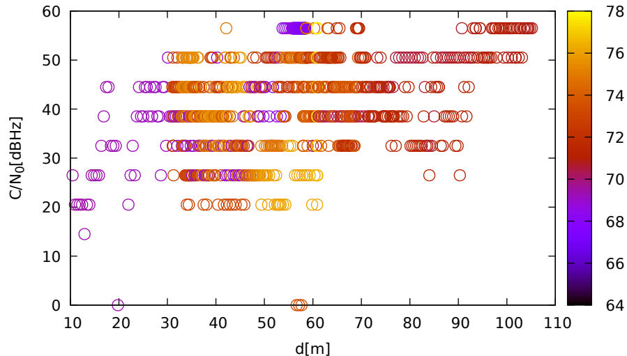
C/N 0 vs distance (LeicaGS15 at C 1 for G01 at L1)
