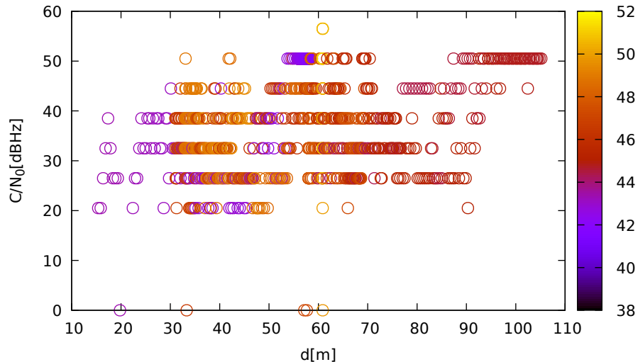
C/N 0 vs distance (LeicaGS15 at C 1 for G03 at L1)
