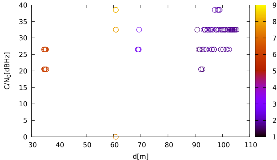
C/N 0 vs distance (LeicaGS15 at C 1 for G04 at L1)
