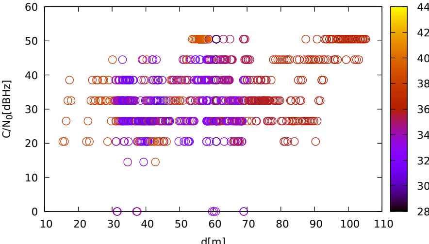
C/N 0 vs distance (LeicaGS15 at C 1 for G08 at L1)
