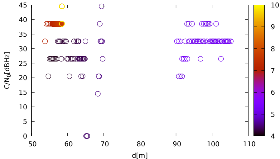
C/N 0 vs distance (LeicaGS15 at C 1 for G10 at L1)
