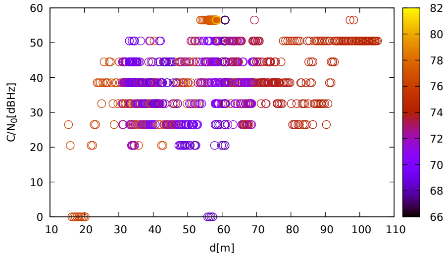
C/N 0 vs distance (LeicaGS15 at C 1 for G11 at L1)
