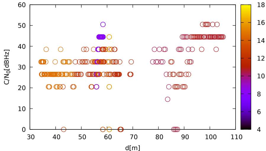
C/N 0 vs distance (LeicaGS15 at C 1 for G17 at L1)
