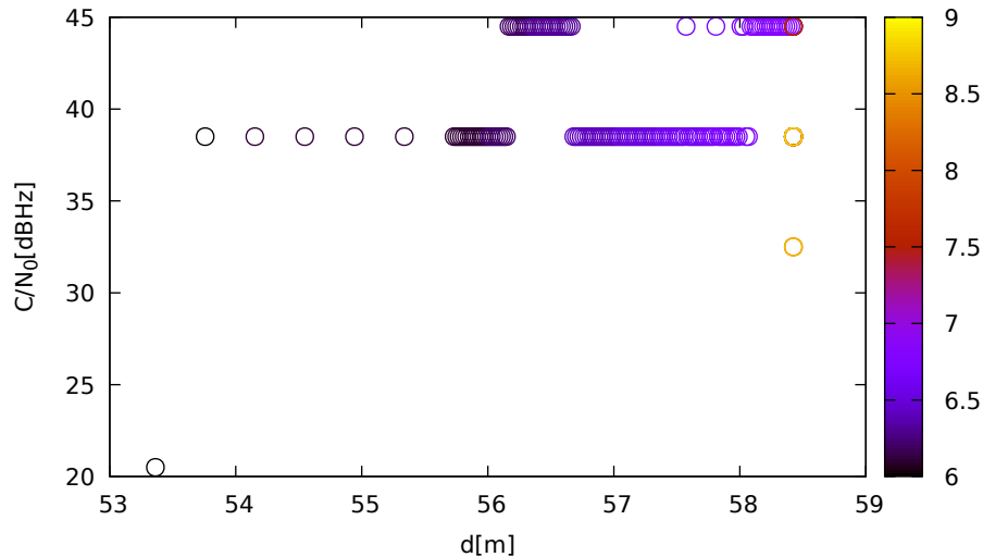
C/N 0 vs distance (LeicaGS15 at C 1 for G21 at L1)
