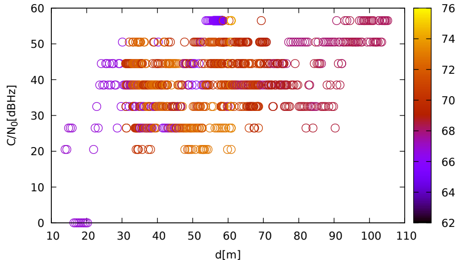
C/N 0 vs distance (LeicaGS15 at C 1 for G22 at L1)
