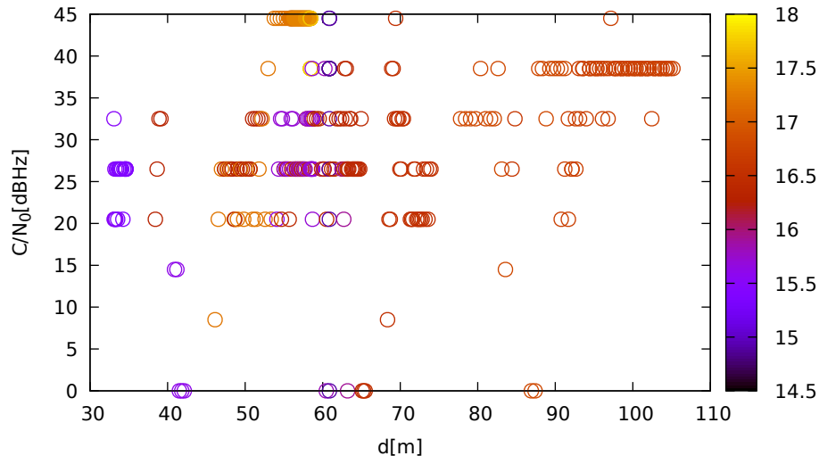
C/N 0 vs distance (LeicaGS15 at C 1 for G28 at L1)
