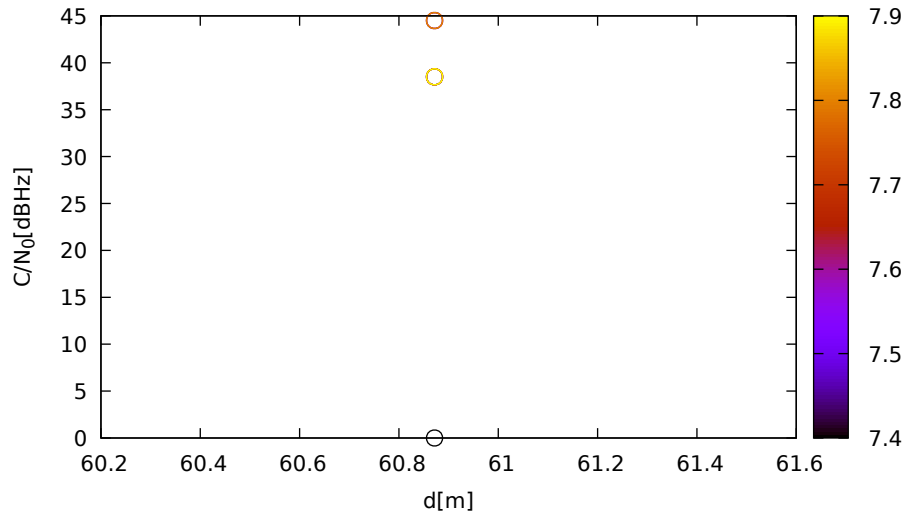
C/N 0 vs distance (LeicaGS15 at C 1 for G31 at L1)
