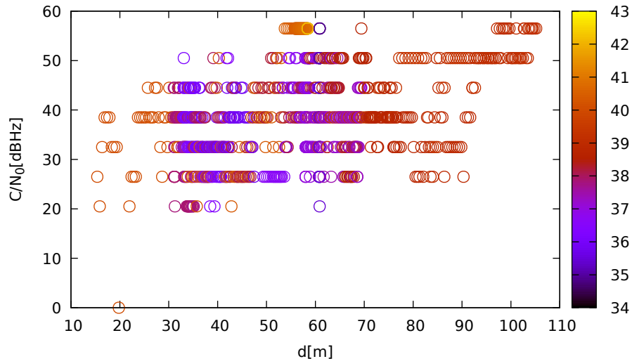
C/N 0 vs distance (LeicaGS15 at C 1 for G32 at L1)
