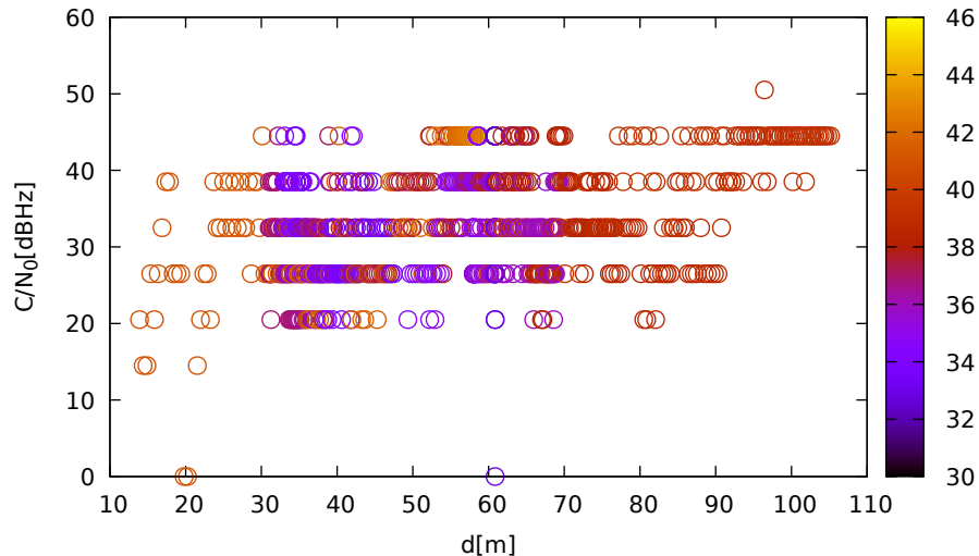
C/N 0 vs distance (LeicaGS15 at C 1 for R06 at L1)
