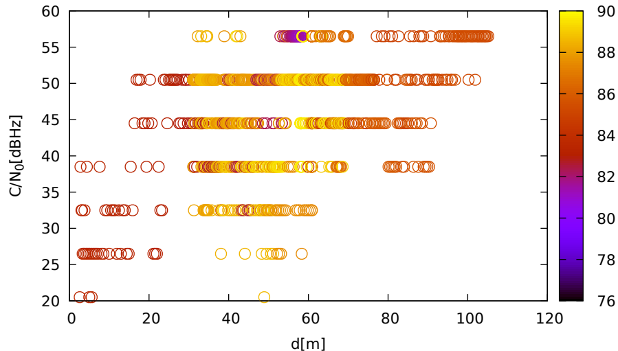
C/N 0 vs distance (LeicaGS15 at C 1 for R07 at L1)
