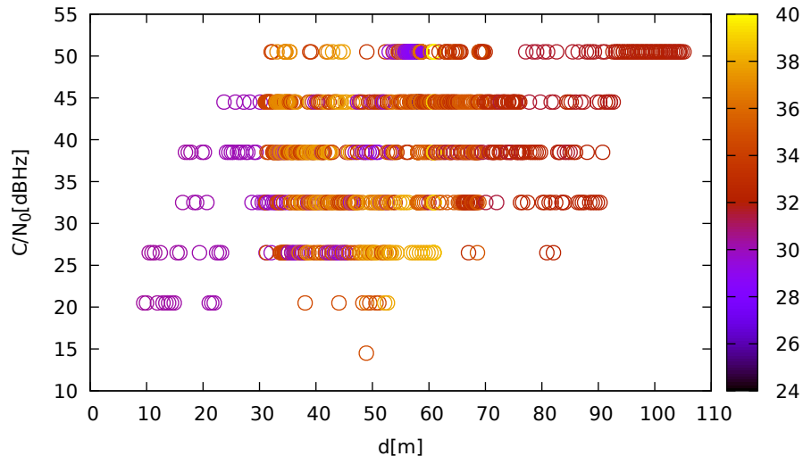
C/N 0 vs distance (LeicaGS15 at C 1 for R08 at L1)
