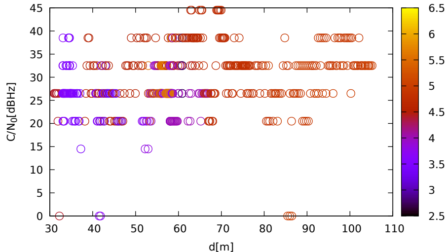
C/N 0 vs distance (LeicaGS15 at C 1 for R14 at L1)
