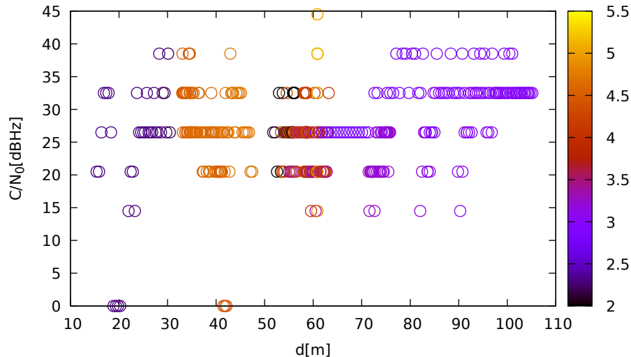
C/N 0 vs distance (LeicaGS15 at C 1 for R15 at L1)
