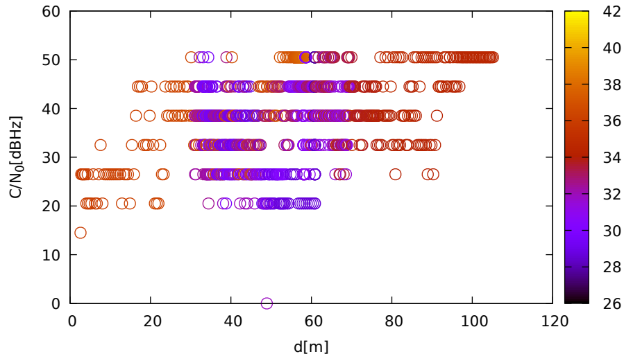
C/N 0 vs distance (LeicaGS15 at C 1 for R21 at L1)
