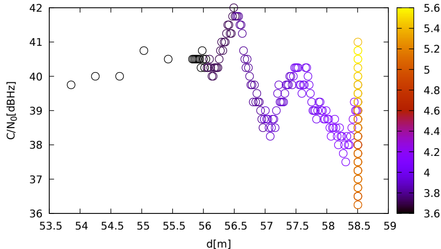
C/N 0 vs distance (LeicaGS18 at C 1 for E02 at L1)
