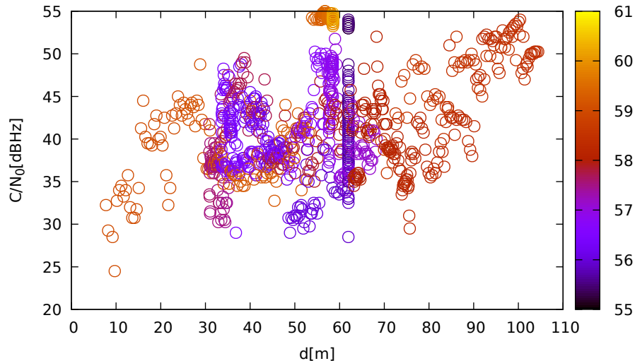
C/N 0 vs distance (LeicaGS18 at C 1 for E04 at L1)
