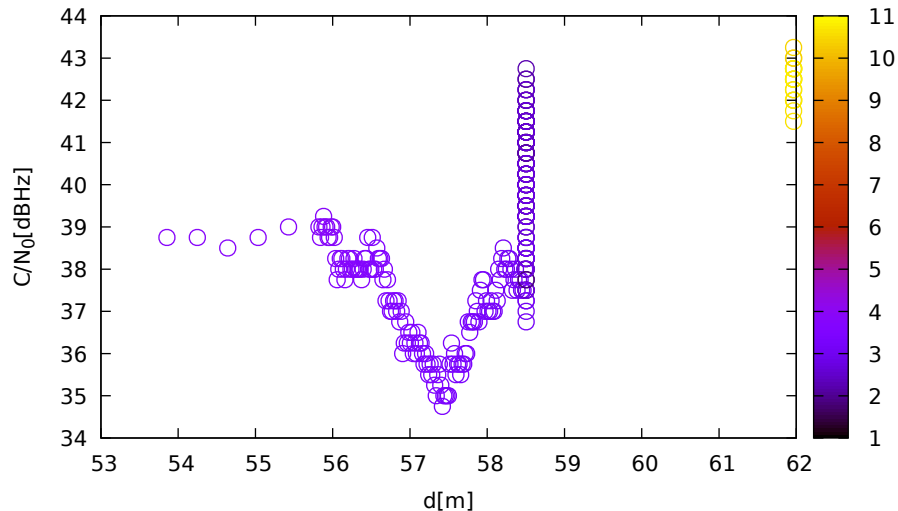
C/N 0 vs distance (LeicaGS18 at C 1 for E05 at L1)
