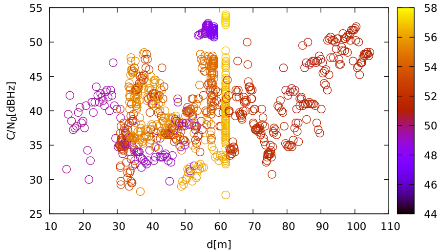
C/N 0 vs distance (LeicaGS18 at C 1 for E09 at L1)
