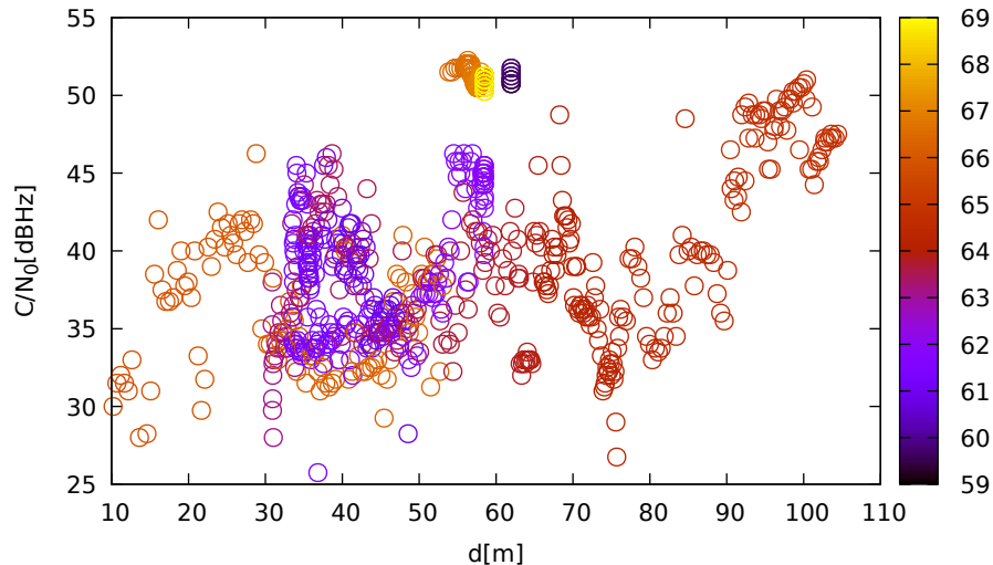
C/N 0 vs distance (LeicaGS18 at C 1 for E11 at L1)
