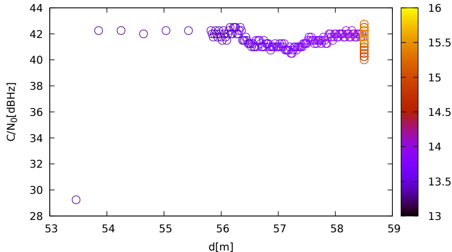
C/N 0 vs distance (LeicaGS18 at C 1 for E12 at L1)
