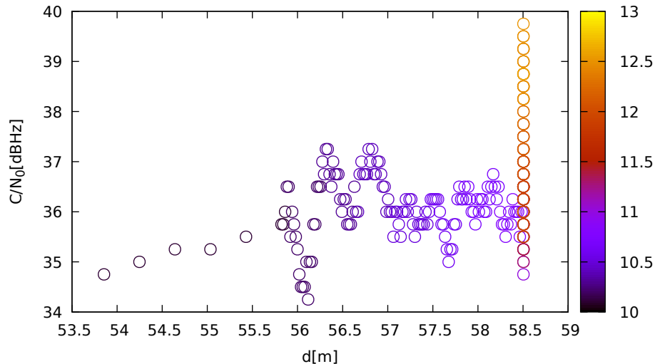
C/N 0 vs distance (LeicaGS18 at C 1 for E19 at L1)
