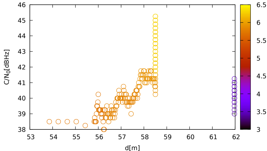
C/N 0 vs distance (LeicaGS18 at C 1 for E30 at L1)
