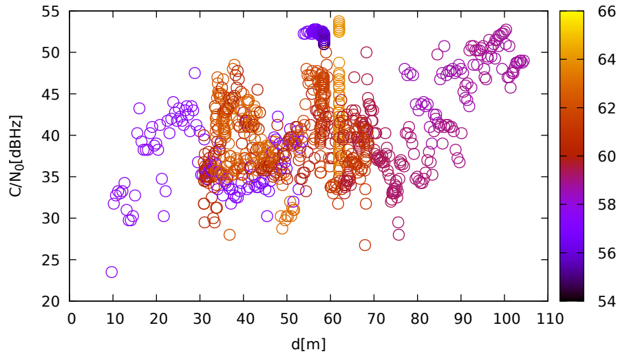
C/N 0 vs distance (LeicaGS18 at C 1 for E36 at L1)
